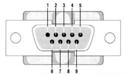
Fig. 2-1 RS-232 pin out DB-9 pin used for Asynchronous Data
