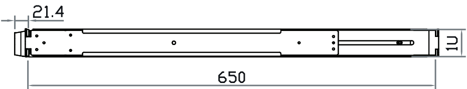
Side View
