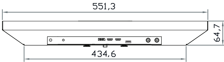
Bottom View
