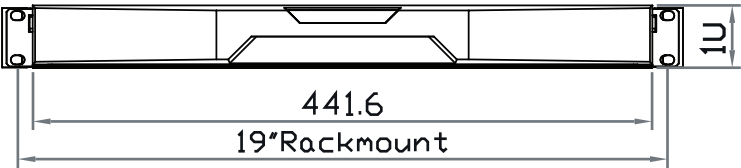
Rear View
