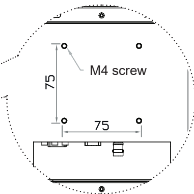
VESA mount ( 75*75mm )
