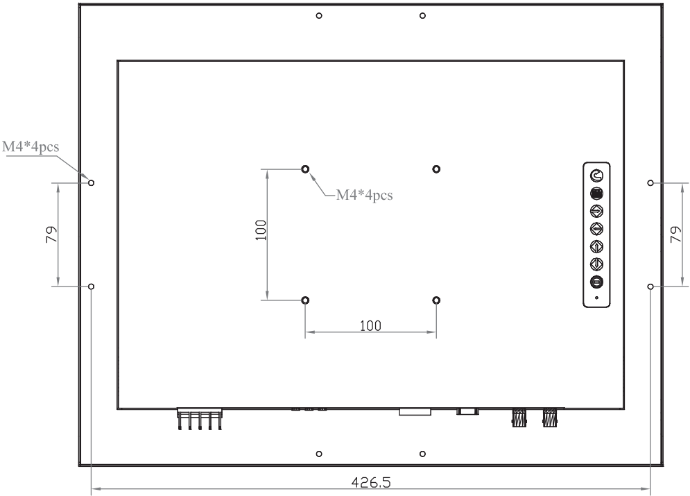
Bottom View
