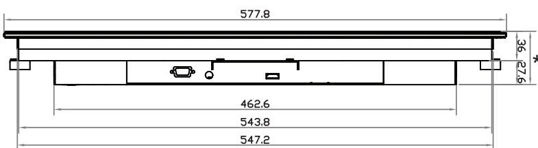
Bottom View
