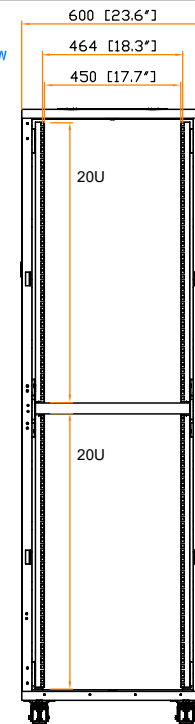
19" rail position
