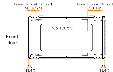
19" rail position
