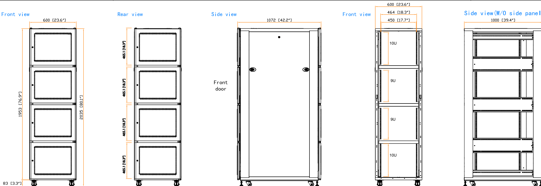
19" rail position
