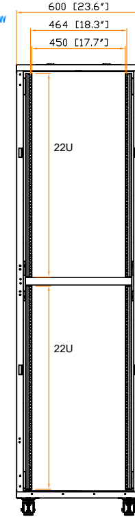
19" rail position
