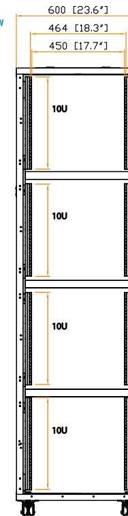
19" rail position
