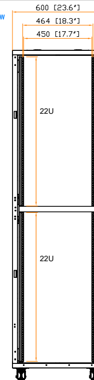
19" rail position
