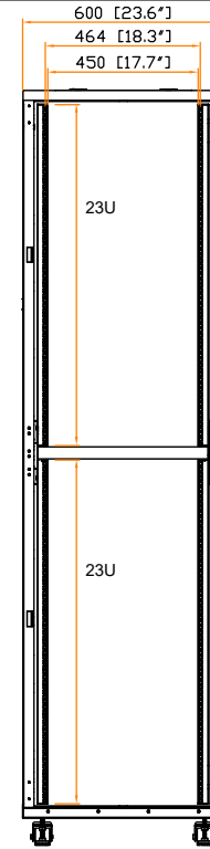
19" rail position
