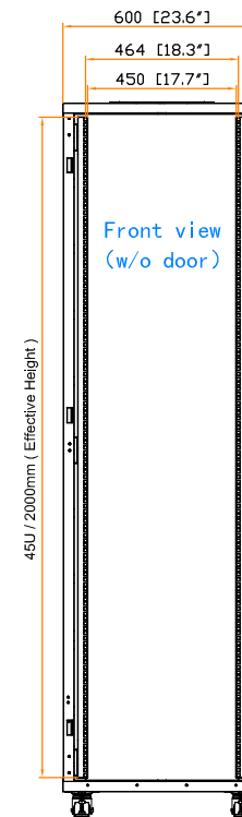
19" rail position
