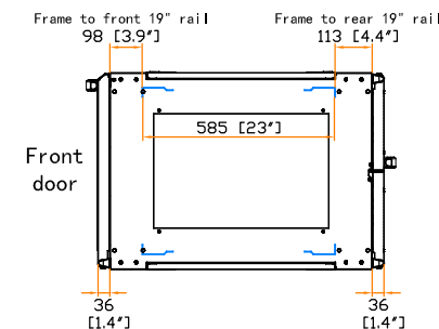
19" rail position
