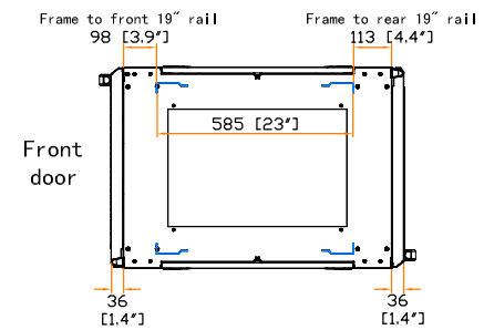
19" rail position
