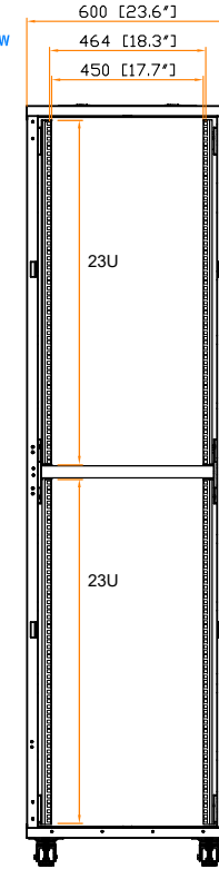
19" rail position
