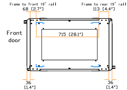
19" rail position
