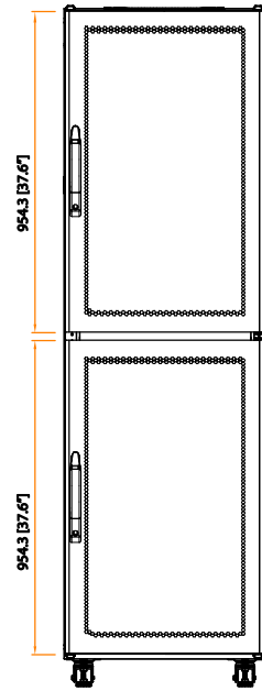
Rear view
