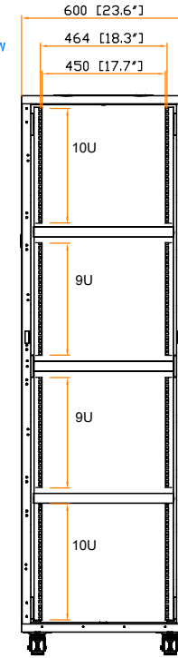
Front view
