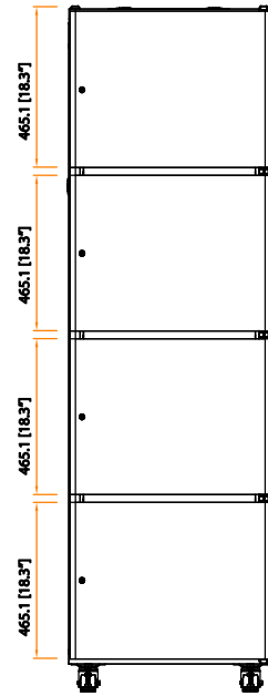
Rear view
