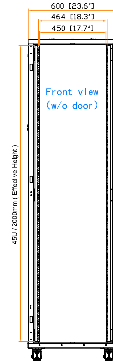
19" rail position
