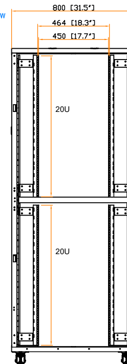
19" rail position
