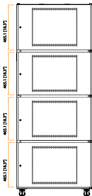
Rear view
