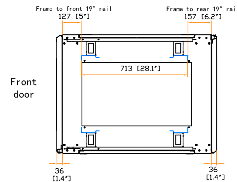
19" rail position
