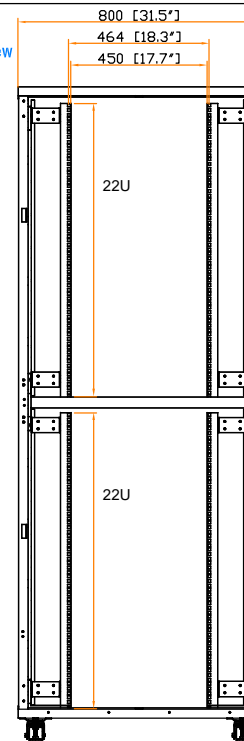
19" rail position
