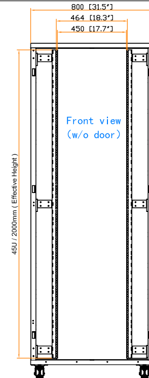
19" rail position
