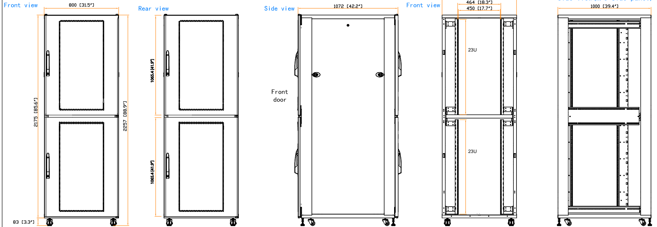
19" rail position
