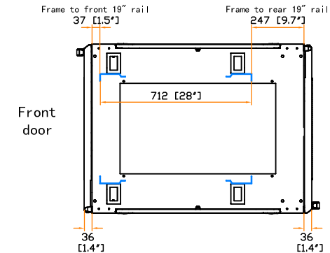
19" rail position
