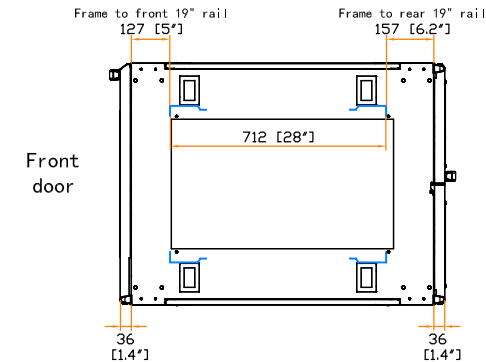
19" rail position
