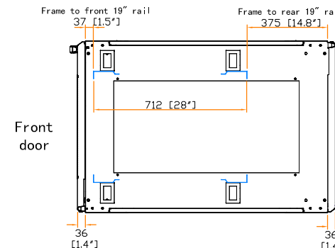
19" rail position
