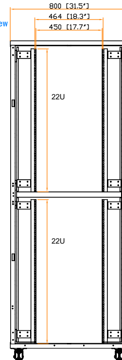
19" rail position
