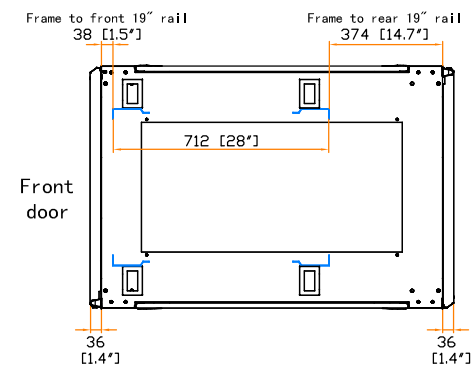
19" rail position
