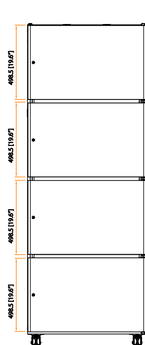
Rear view
