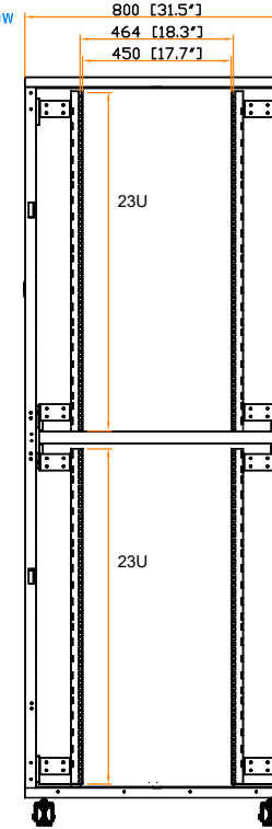
19" rail position
