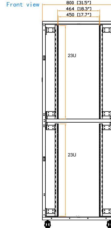
19" rail position
