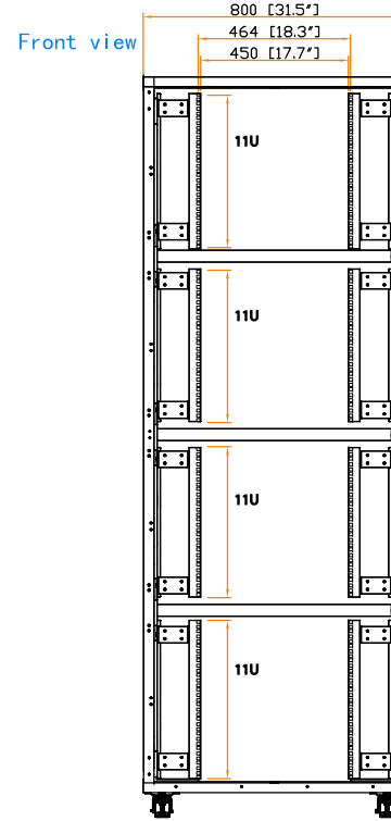
19" rail position
