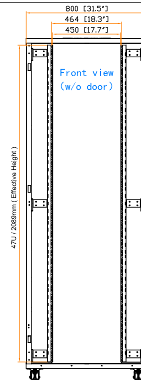
19" rail position
