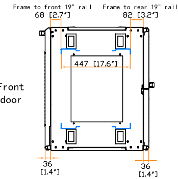
19" rail position
