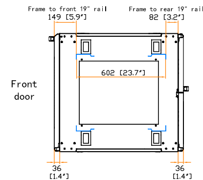
19" rail position
