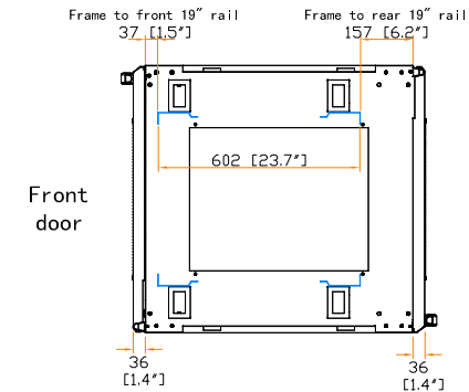
19" rail position
