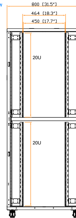
Front view
