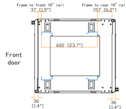
19" rail position
