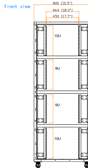
19" rail position
