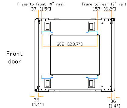
19" rail position
