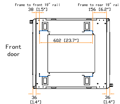
19" rail position
