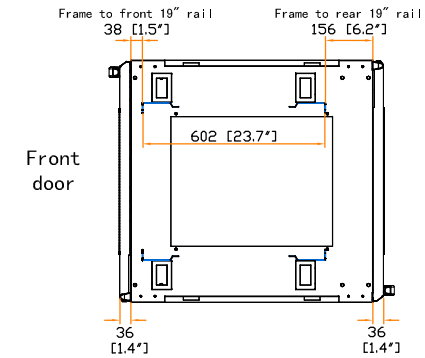
19" rail position
