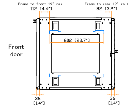
19" rail position
