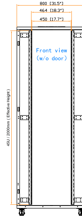
19" rail position
