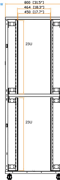
19" rail position
