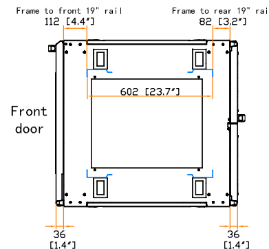
19" rail position
