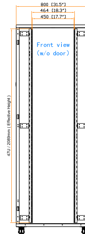
19" rail position
