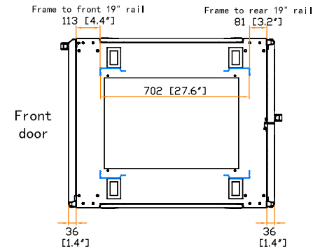
19" rail position
