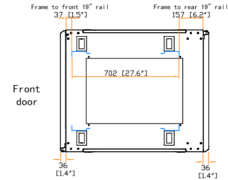
19" rail position
