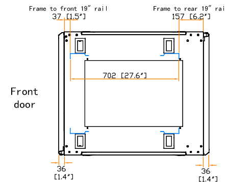
19" rail position
