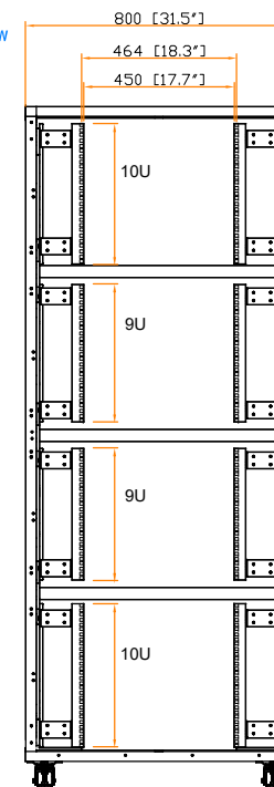
19" rail position
