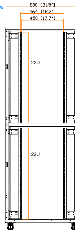
19" rail position
