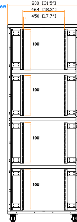
19" rail position
