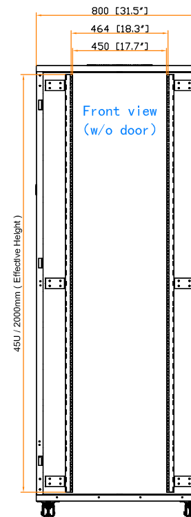
19" rail position
