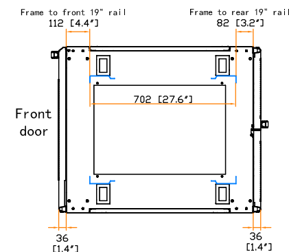
19" rail position
