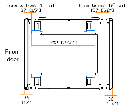
19" rail position
