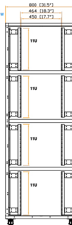
19" rail position
